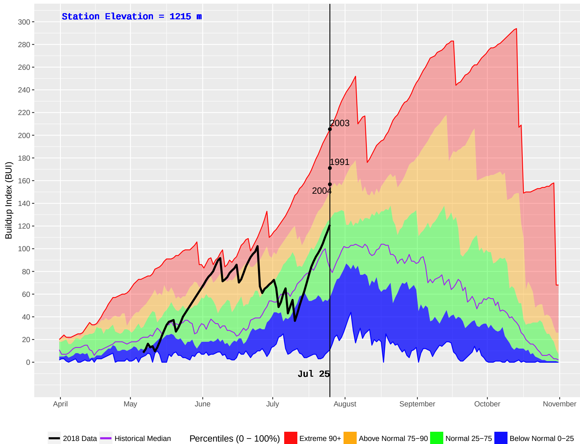
ALLISON PASS (317) : Historical (1987–2016) and Current (2018) Noon Buildup Index (BUI)
