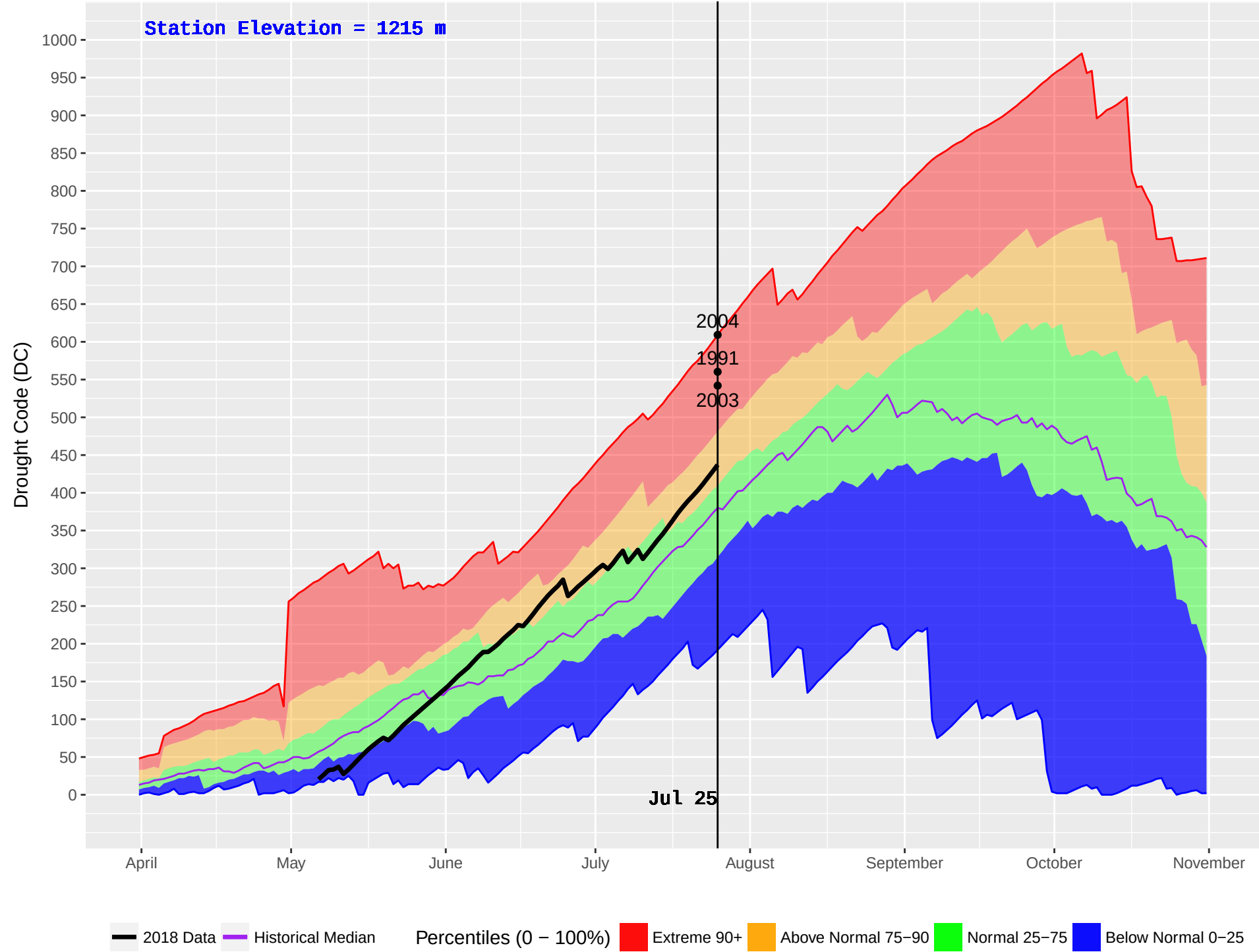
ALLISON PASS (317) : Historical (1987–2016) and Current (2018) Noon Drought Code (DC)
