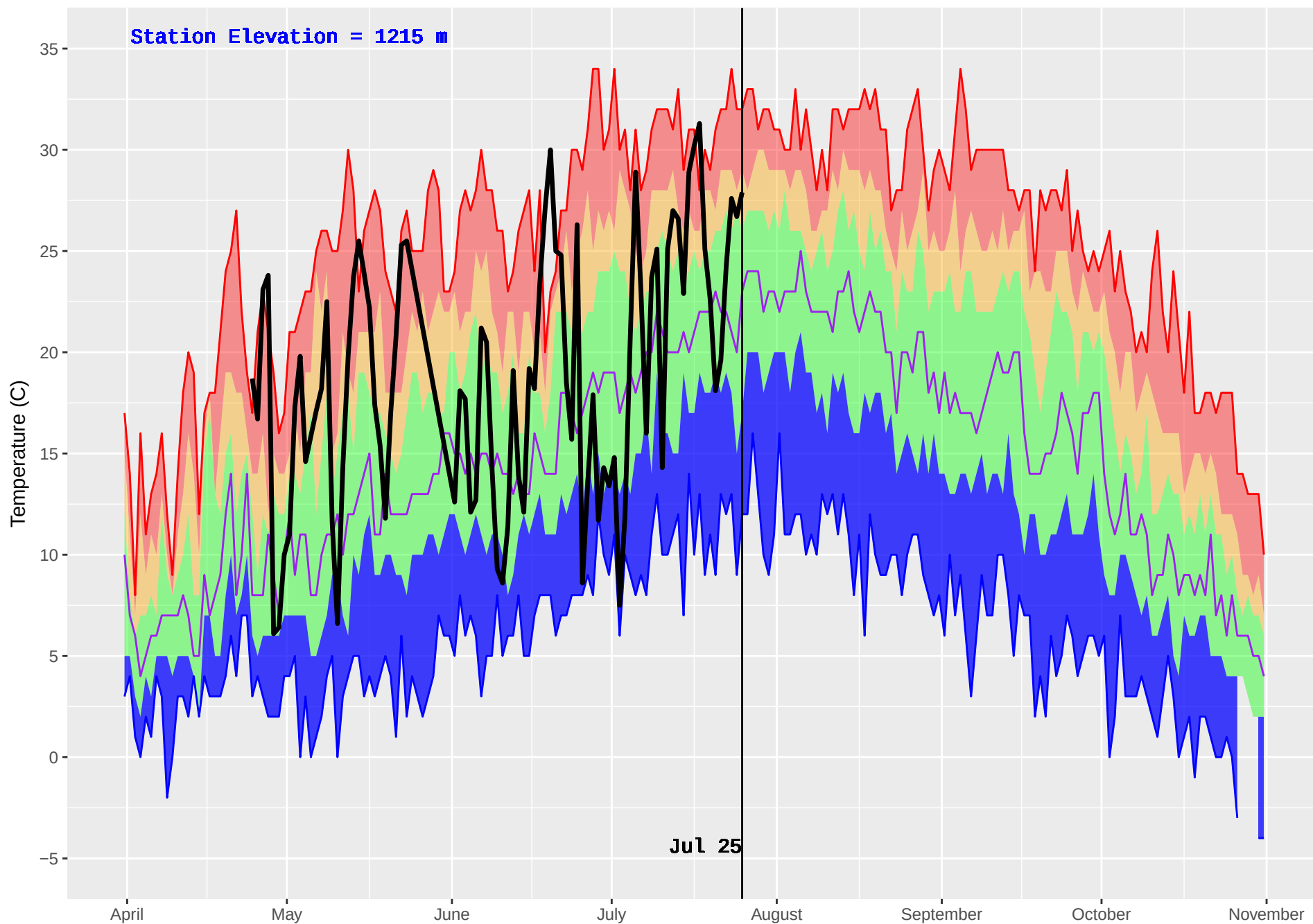
ALLISON PASS (317) : Historical (1987–2016) and Current (2018) Noon Temperature
